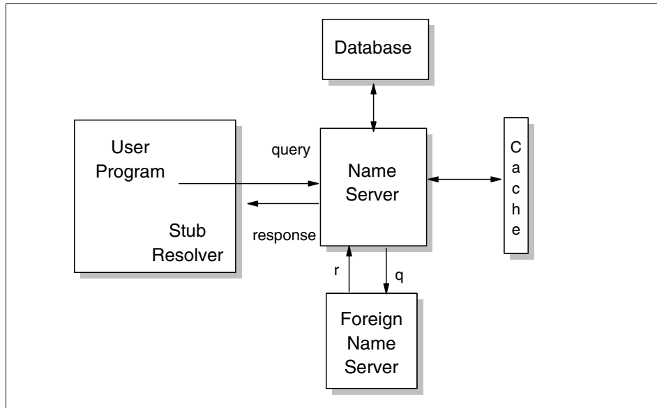
Figure 12-3 DNS: Using a stub resolver for domain name resolution
