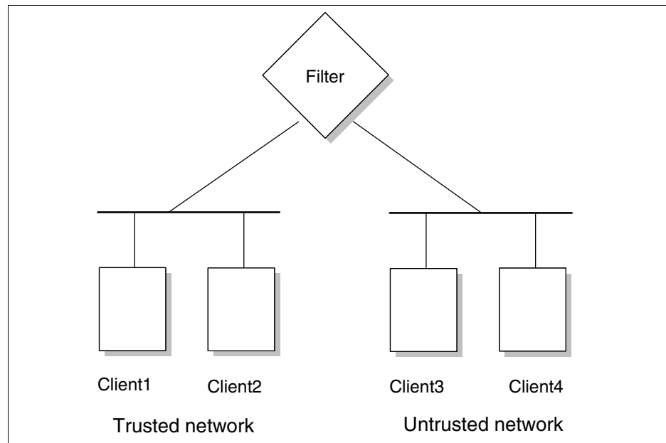
Figure 22-12 Packet-filtering router
