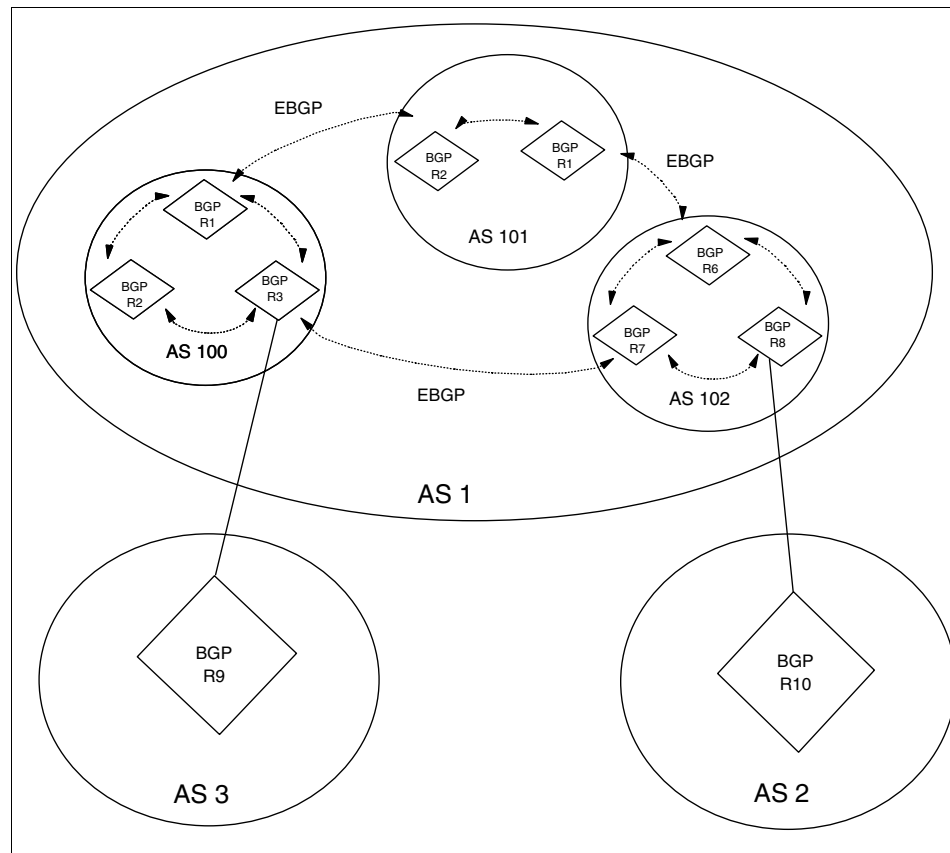
Figure 5-28 BGP confederations
