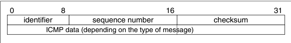
Figure 3-27 ICMP: Message format
