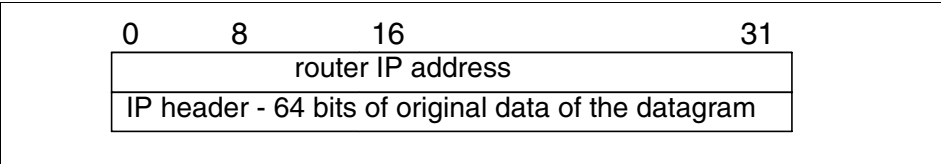
Figure 3-32 ICMP: Redirect
