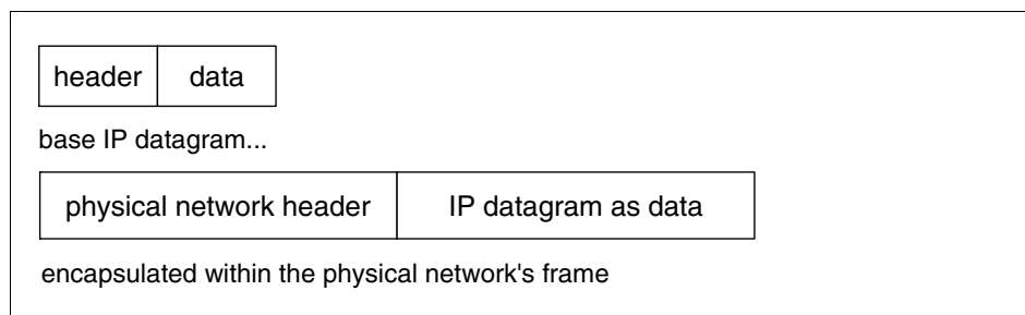
Figure 3-16 IP: Format of a base IP datagram
